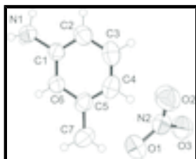
Fig. 1. The asymmetric unit of the title compound showing the atomic numbering scheme. Displacement ellipsoids are shown at the 50% probability level.
