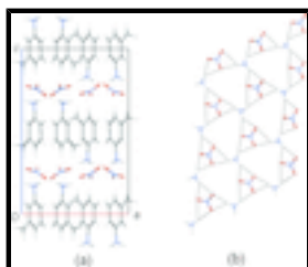
Fig. 2. (a) Packing diagram of the title compound viewed down the b -axis. (b) N—H...O hydrogen bonding network in the title compound (dashed lines indicate hydrogen bonds).
